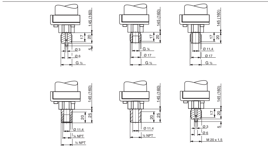
Fig.: 3 Process couplings
