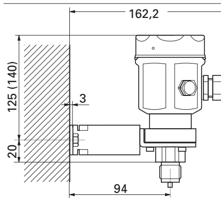
Fig.: 10 Wall mounting
